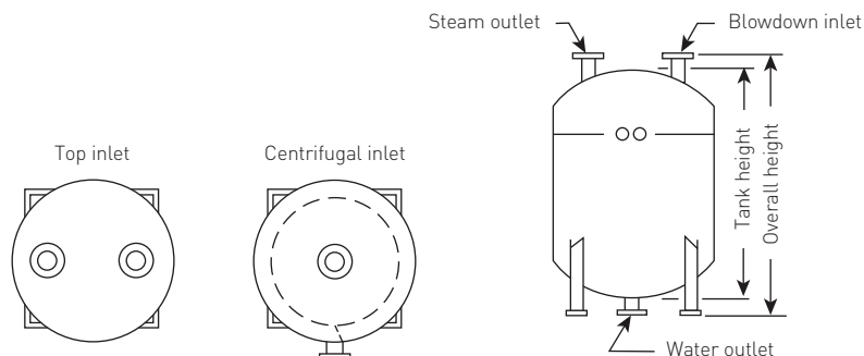
FIGURE 7.6 Sizing top or centrifugal inlet tank
