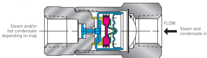
FIGURE 3.11 Bellows trap
