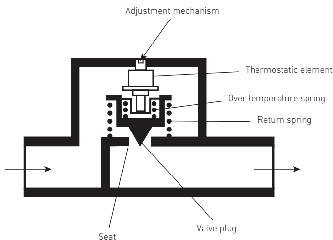
FIGURE 3.12 Wax capsule trap
