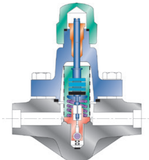
FIGURE 3.10 Bimetallic trap
